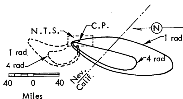
Fig. 1. Fallout from the Turk shot fired in 1955. The solid lines show the predicted fallout pattern; the dotted lines show the actual fallout pattern determined by ground survey. (From Ref. 1.)
